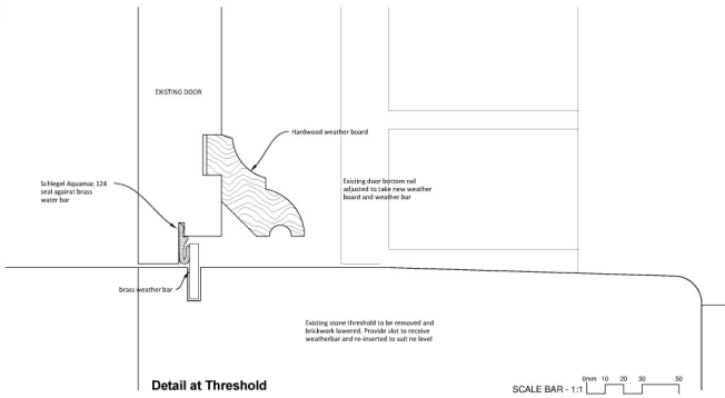
Detail at Threshold
